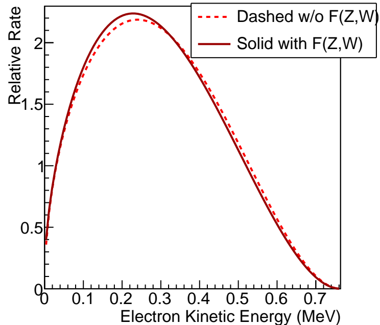
^{204}\text{Ti} Beta Decay Spectrum
