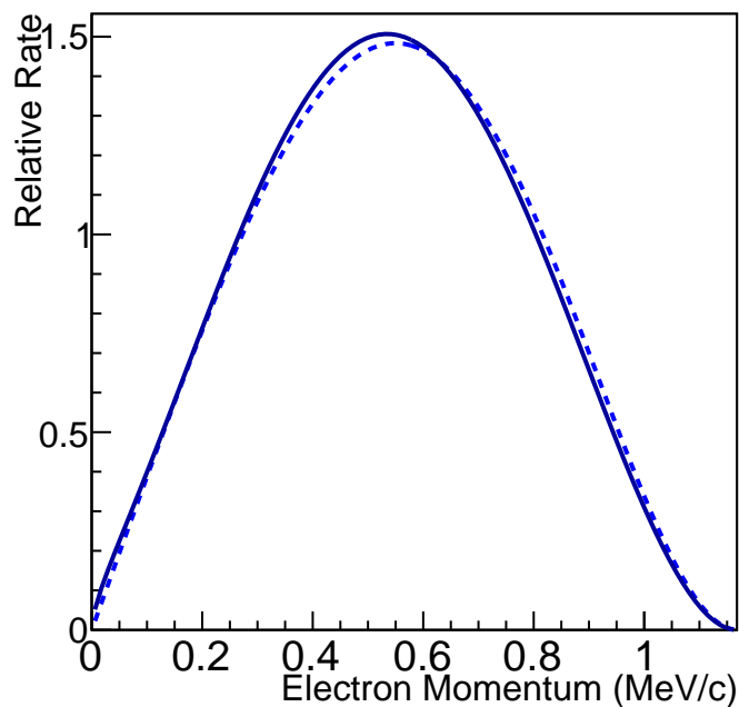
^{204}\text{Ti} Beta Decay Spectrum
